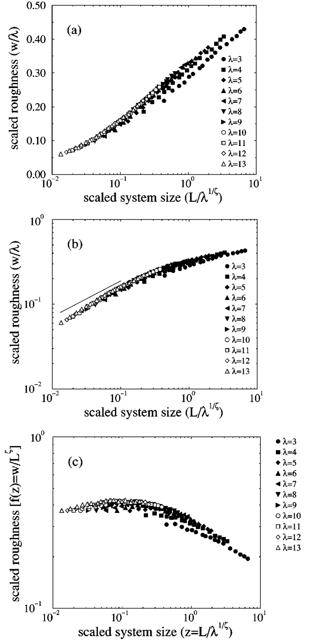
FIG. 4. (a) and (b) The data collapse, w/\lambda vs L/\lambda^{1/\zeta} , \zeta = \zeta_{\text{RB}} = 0.42 , for the roughness of (2+1) -dimensional \{100\} oriented systems. The random bonds are from uniform distribution with \Delta J_{ij,\perp}/J_0 = 1 in the perpendicular ( z ) direction and constant J_{ij,\parallel}/J_0 = 0.2 in the parallel ( x, y ) direction. The number of realizations N = 200 for each wavelength \lambda \in [3, \dots, 13] and system size L^3 \in [6^3 - 90^3] . (c) The scaling function f(z) = w/L^\zeta of the roughness w(L, \lambda) vs scaling parameter z = L/\lambda^{1/\zeta} . Finite-size effects with logarithmic corrections are visible as a curvature for small L .
